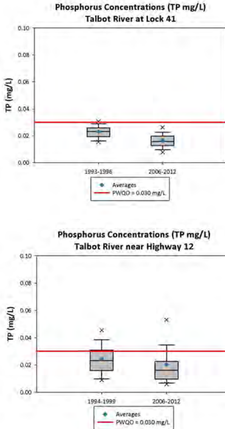
Figure 4-3: Total phosphorous concentrations at the two Talbot River LSPP monitoring sites.
