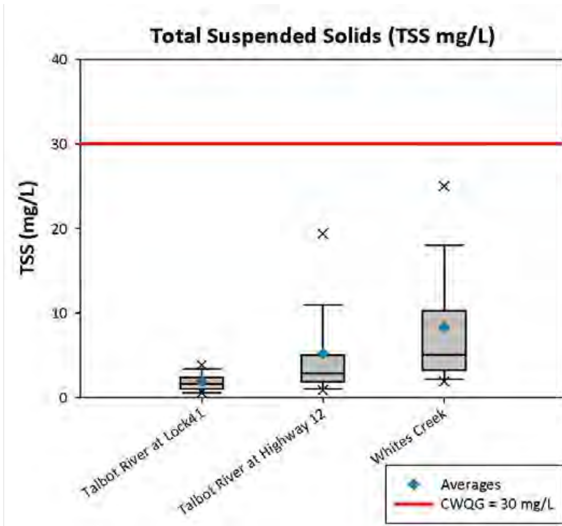
Figure 4-8: Total suspended solids concentrations in the Talbot River and Whites Creek subwatersheds
