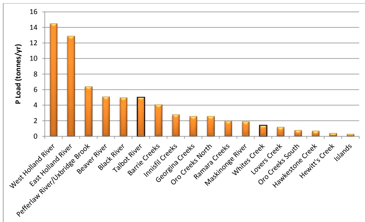
Figure 4-9: Average phosphorus loads (tonnes/year) contributed by each Lake Simcoe subwatershed (data: LSRCA/MOEC, 2013)
