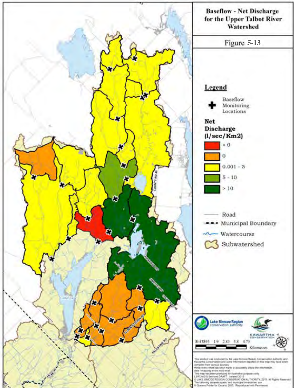
Figure 5 - 13: Baseflow Distribution in the Upper Talbot Watershed
