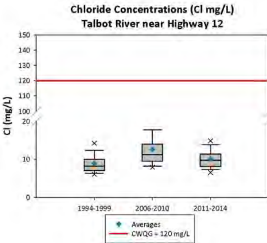
Figure 4-5: Chloride concentrations in the Talbot River subwatershed.
