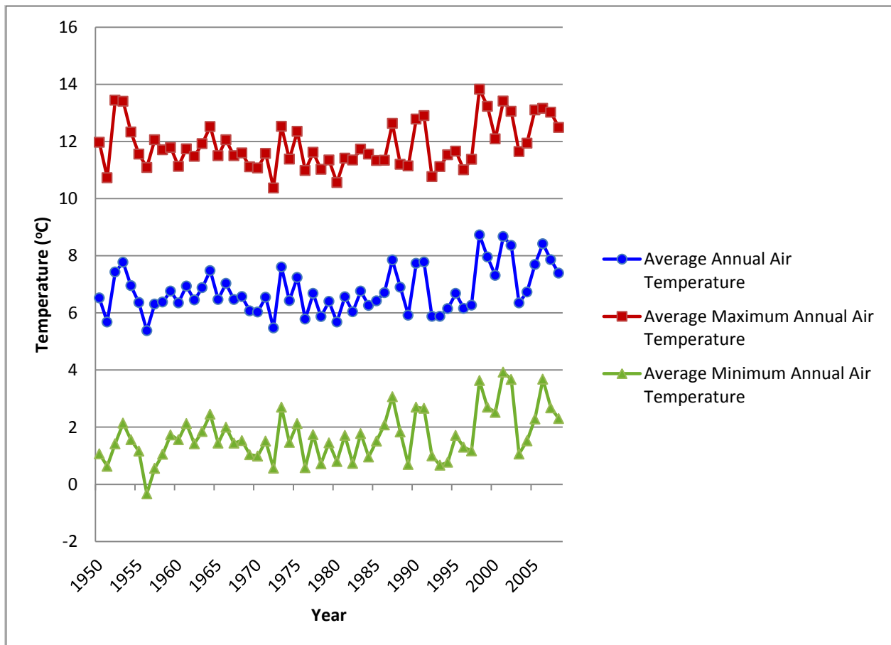
Figure 3- 12: Comparison of the average annual, maximum and minimum temperatures at the Barrie WPCCC Meteorological Monitoring Station (1950-2008). Source: SGBLS, 2012.
