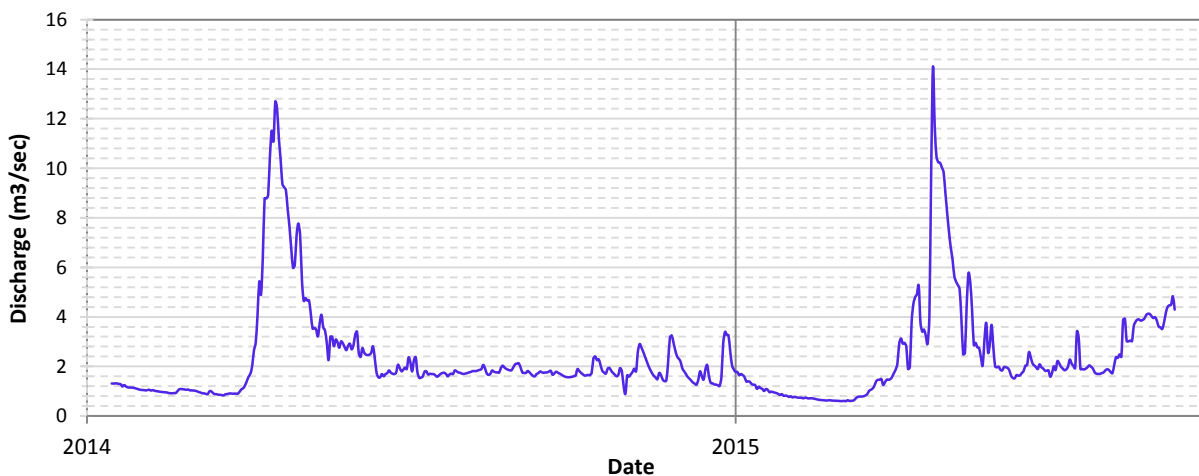
Figure 5 - 18: Mean daily discharge observed at Talbot River at Kirkfield Rd.
