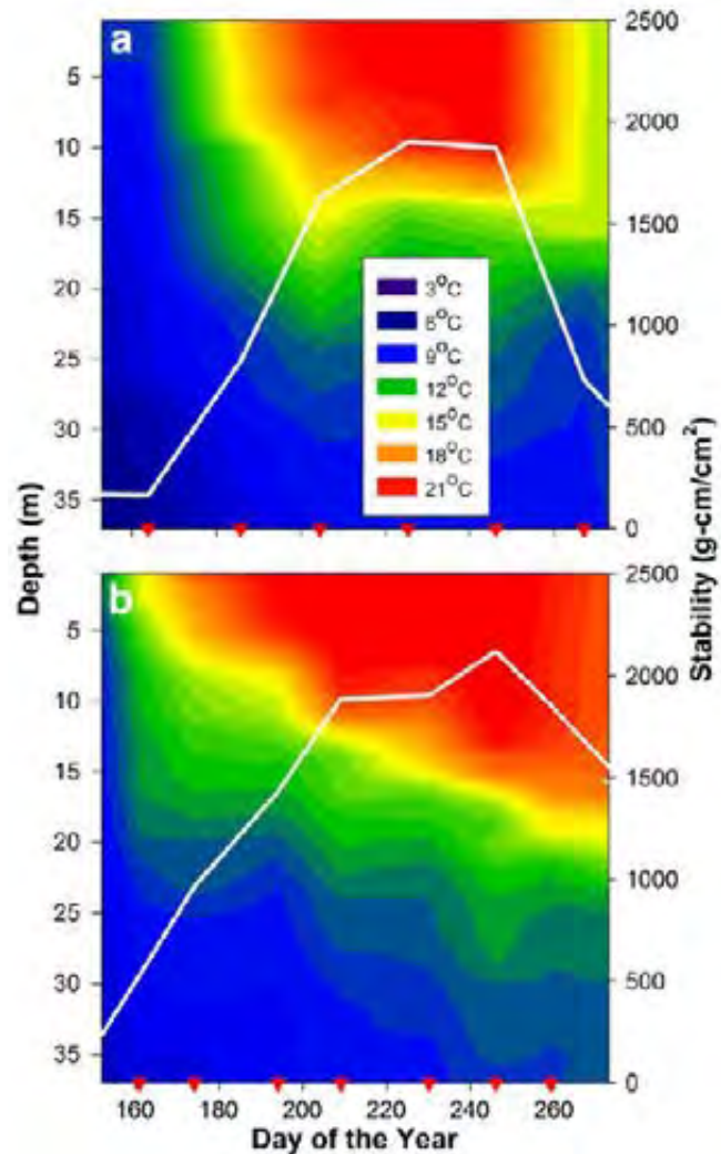
Figure 3- 16: Seasonal water column temperature contour (in degrees Celsius) and stability (white line) in Kempenfelt Bay in 1980 (a) and 2002 (b). Red triangles show the sampling dates along the x-axis. Source: Stainsby et al. , 2011
