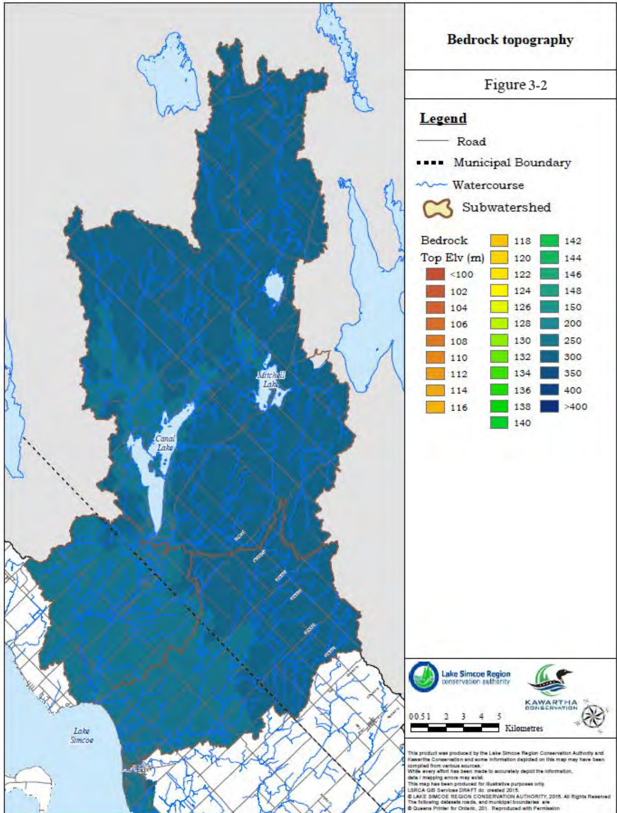
Figure 3-2: Bedrock topography in the Whites Creek and Talbot River subwatersheds.
